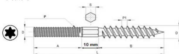
Hanger bolt with Hexagonal Passage, TX25, Zn
