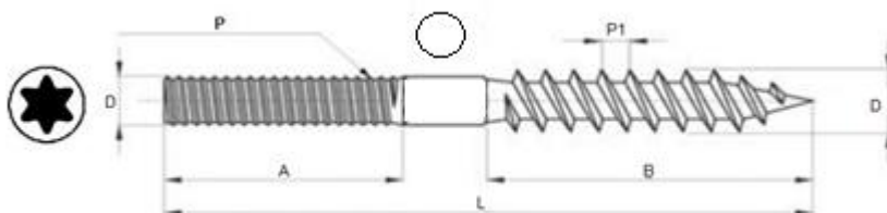
Hanger bolt without Hexagonal Passage, TX15, Zn
