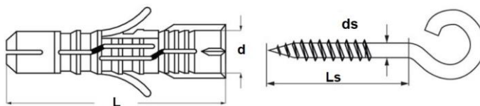
PP Multi Plug with C-Hook PCH
